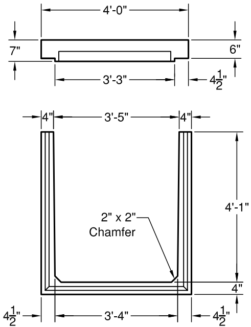
ELEVATION AA
