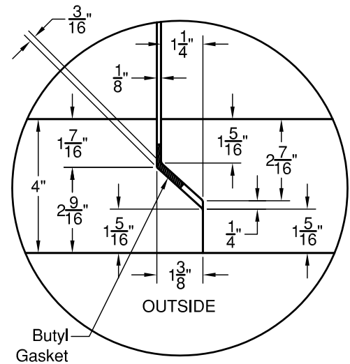
ELEVATION AA
