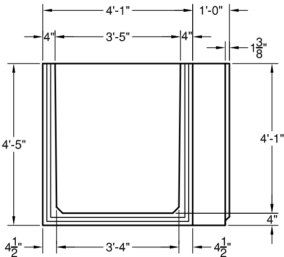
ELEVATION AA
