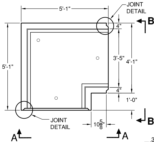
PLAN
