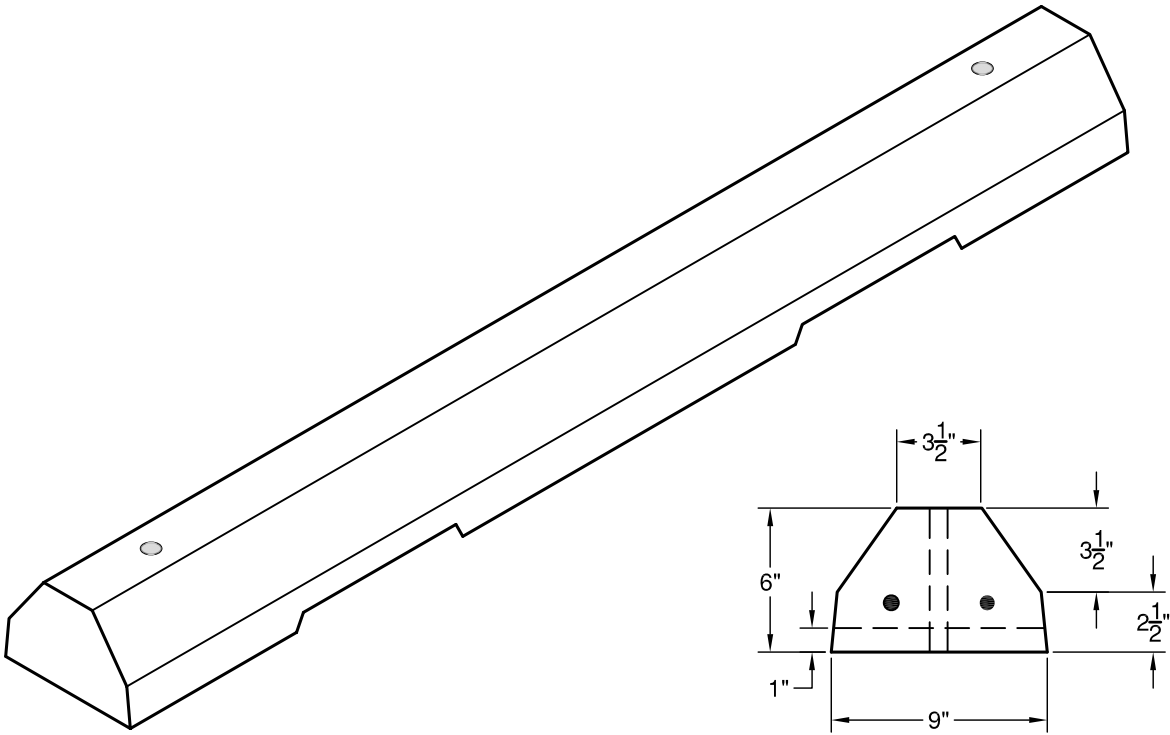
SECTION
