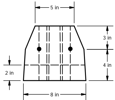
SECTION A-A SCALE 1 / 6
