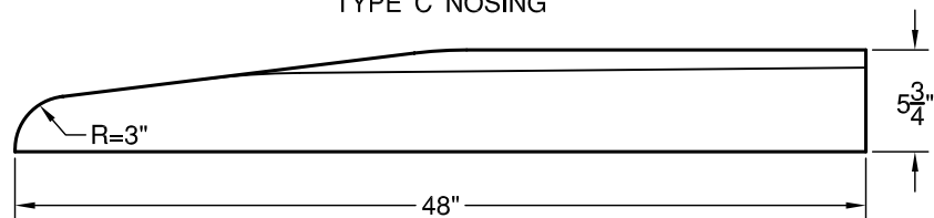
PLAN TYPE 'C' NOSING
