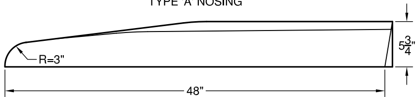
ELEVATION TYPE 'A' NOSING
