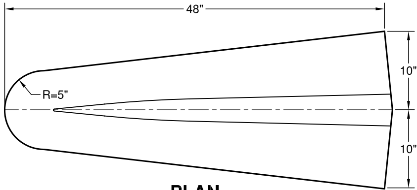
PLAN TYPE 'A' NOSING
