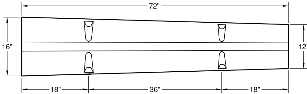
TYPE 'A' CONNECTING DIVIDER No.1
