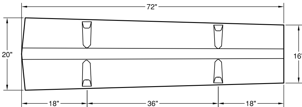
TYPE 'A' CONNECTING DIVIDER No. 2
