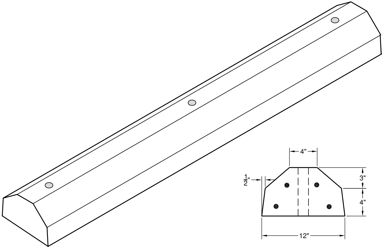
SECTION
