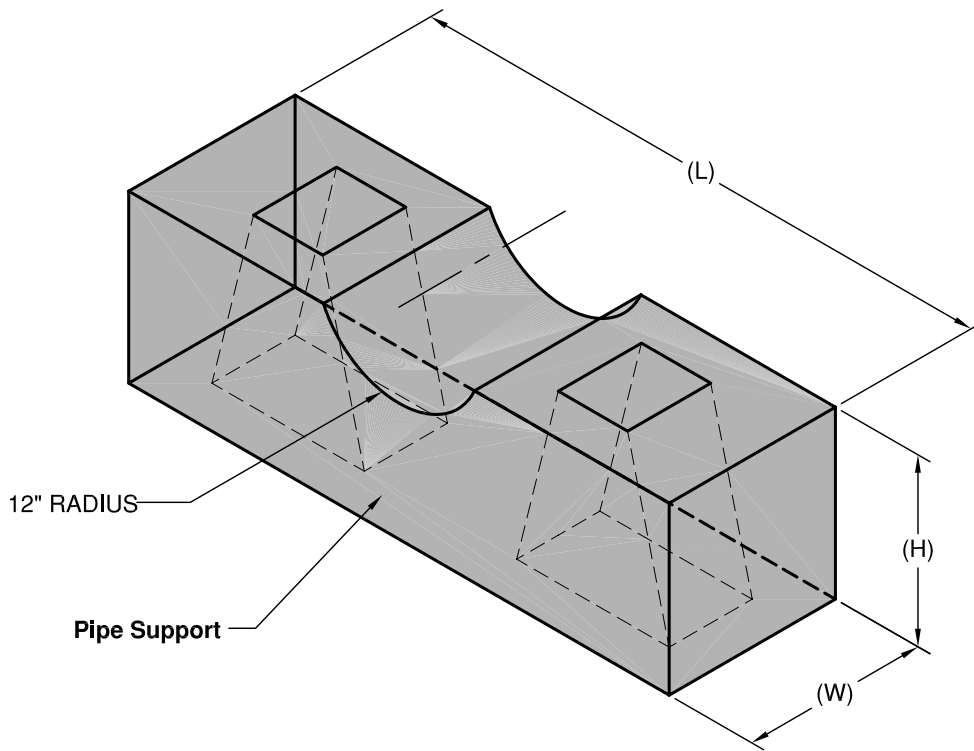
ISOMETRIC REPRESENTATION
