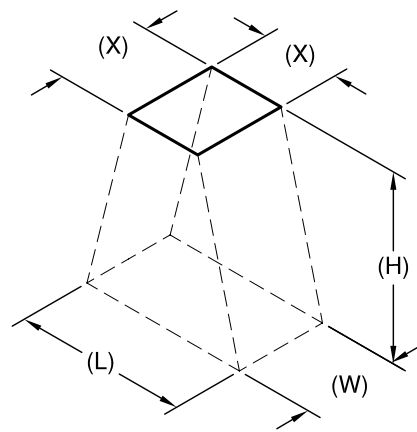
OPTIONAL VOID FOR PILING SUPPORT
