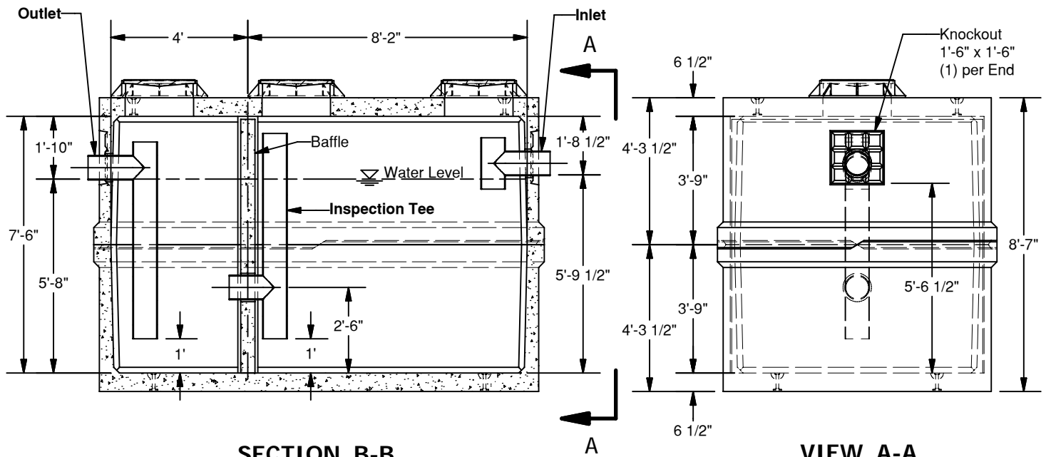
SECTION B-B
