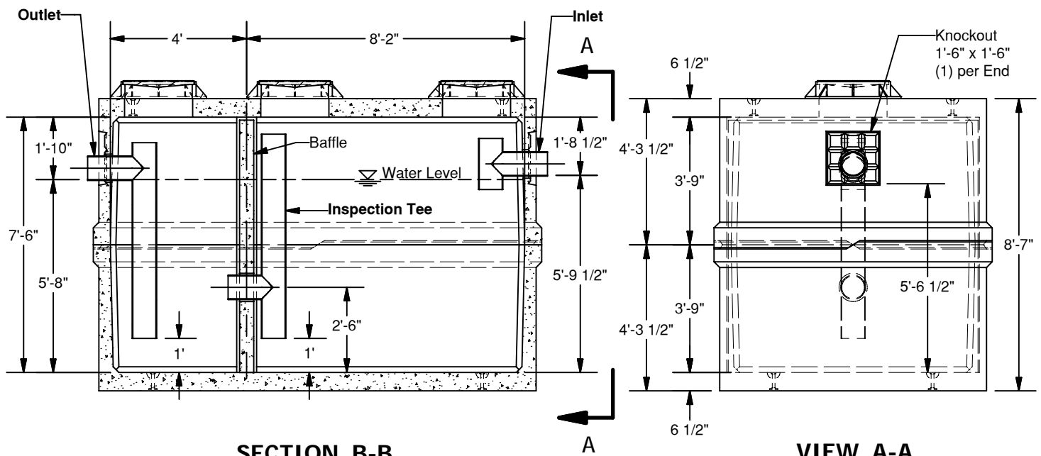
SECTION B-B
