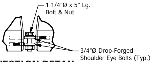
CONNECTION DETAIL
