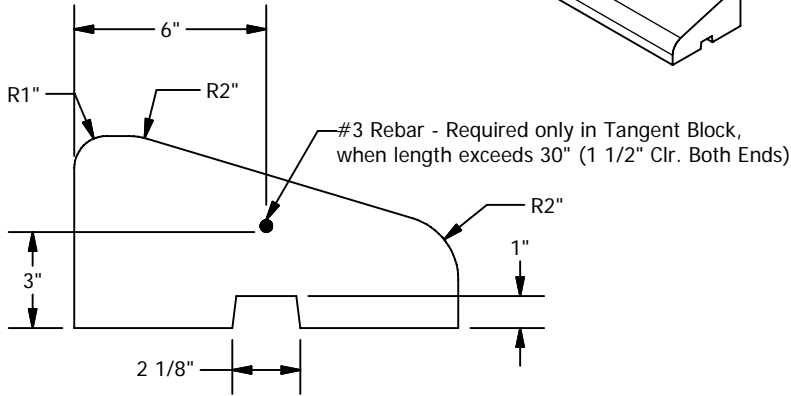
END VIEW
