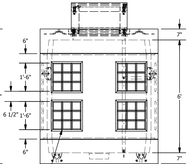
END VIEW
